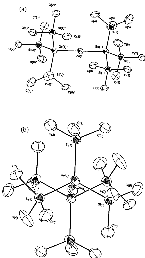
Fig. 1. An ORTEP representation of bis[(tris(trimethylsilyl)germyl)zinc] 1 (hydrogen atoms are omitted for clarity).
